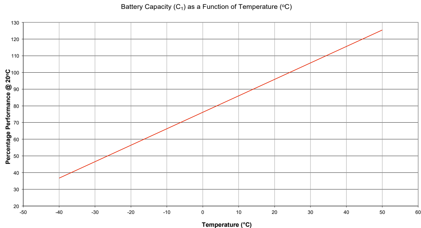
Figure 2 - Battery capacity as a function of temperature
