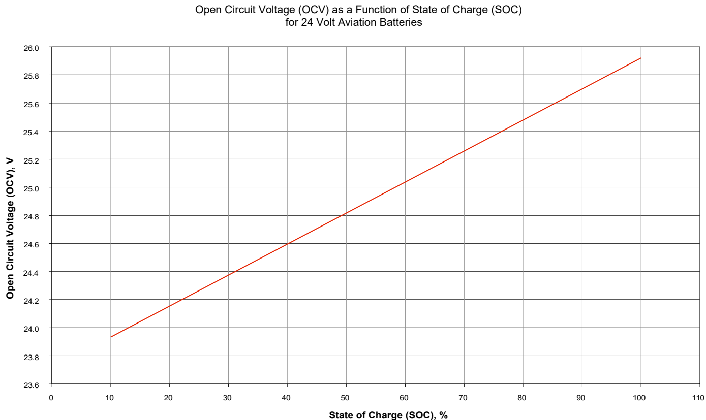
Figure 3 - Open circuit voltage as a function of state of charge
